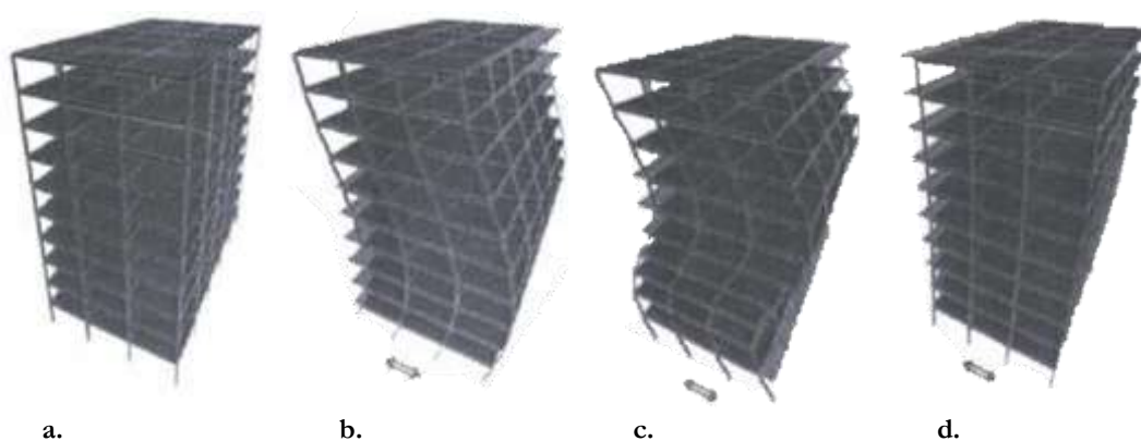
Fig. 1. Modal polyhedron of a 10-story building; a. mode 1, b. mode 2, c. mode 3, d. mode 4.
