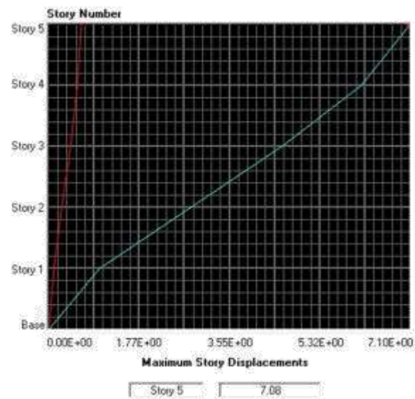
Fig. 2. Maximum displacement of floors (in centimetres) under load - EPX model 5T [13].
