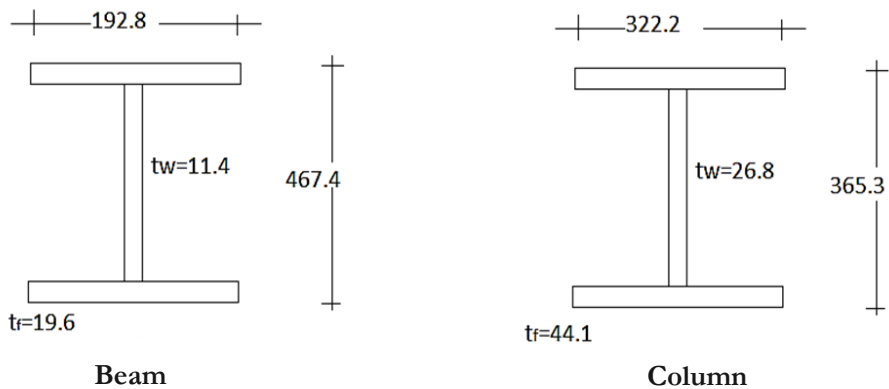
Fig. 3. Beam and column cross-sections in millimeters.
