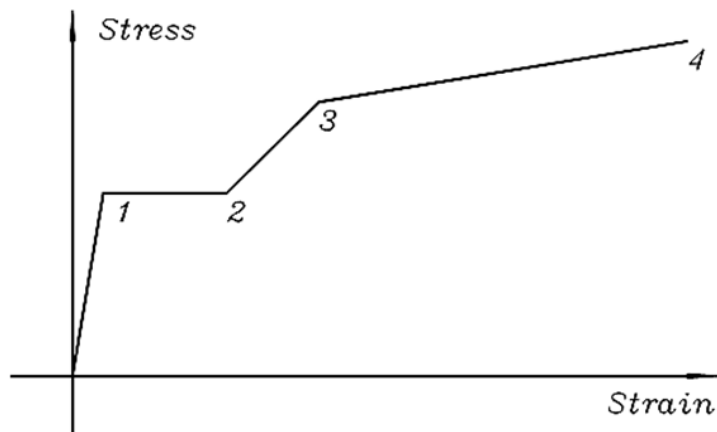
Fig. 2. Stress-strain curve.
