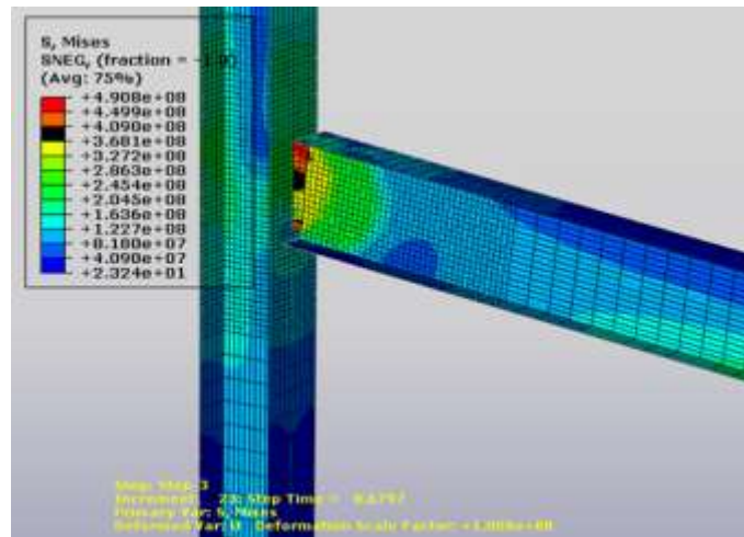
Fig. 6. Stress gauge of the unreinforced model in Abaqus software.
