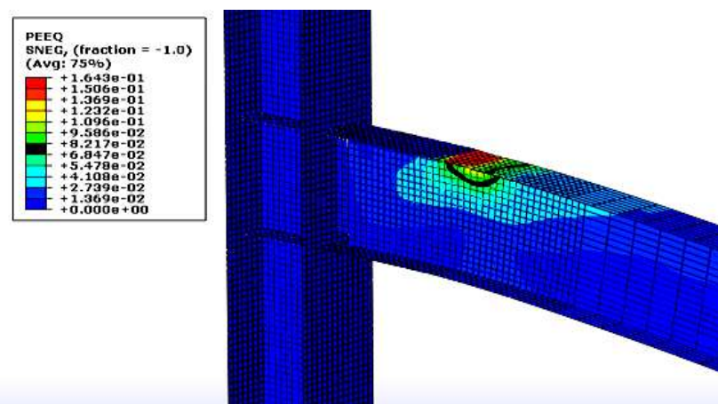
Fig. 8. Shows the plastic strain gauge of the reinforced model when the displacement on the right side of the beam is 1.1 m.
