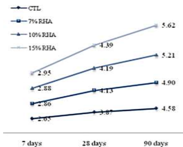
Fig. 5. Results of the tensile strength test of concrete containing rice husk ash.
