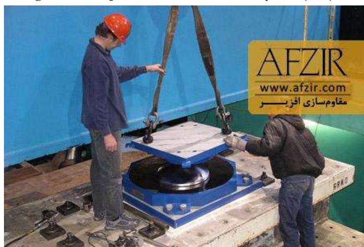
Fig. 4. Installation of pendulum separators.
