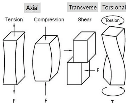
Fig. 3. Four kinds of static loads [51].
