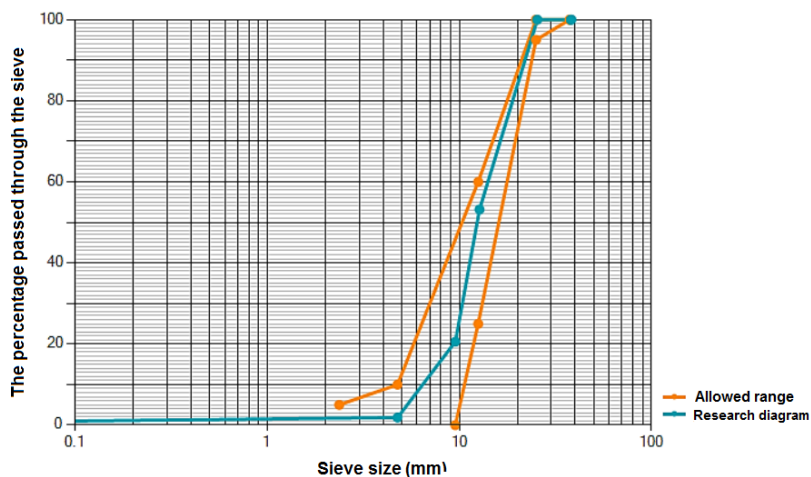
Fig. 1. The training curve of the sand used in the research compared to the permissible limits of ASTM.
