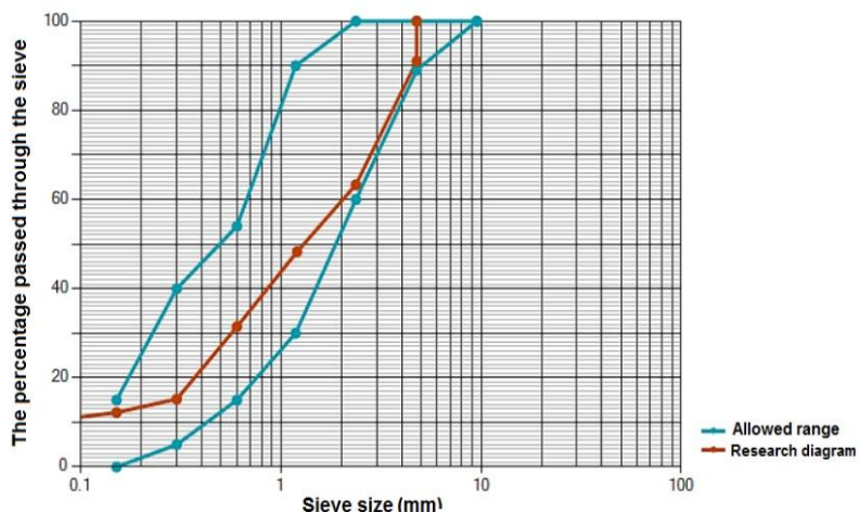
Fig. 2. The graining curve of the sand used in the research is compared to the permissible limits of ASTM.
